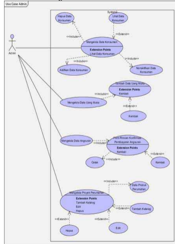
Gambar 4. Use Case Diagram Halaman Admin
