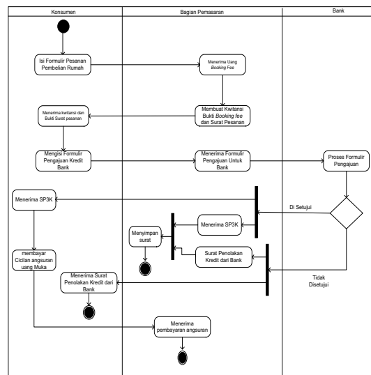
Gambar 2. Activity Diagram Pengajuan Kredit
