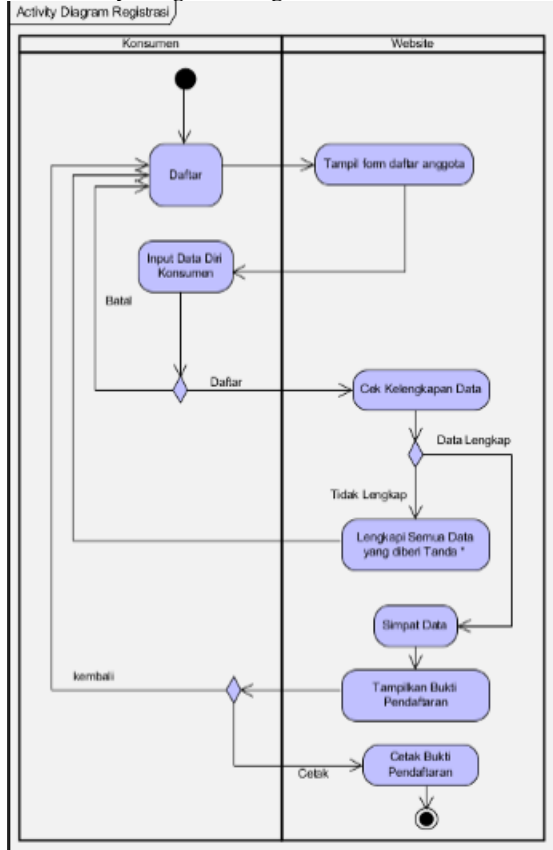
Gambar. 6 Activity Diagram registrasi
