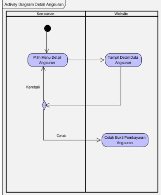
Gambar.7 Activity Diagram Data detail Angsuran
